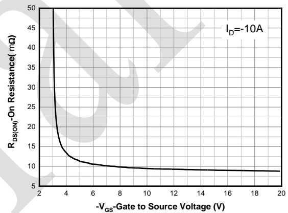
On-Resistance vs. Gate-to-Source Voltage (4)
