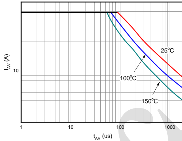
Avalanche characteristics
