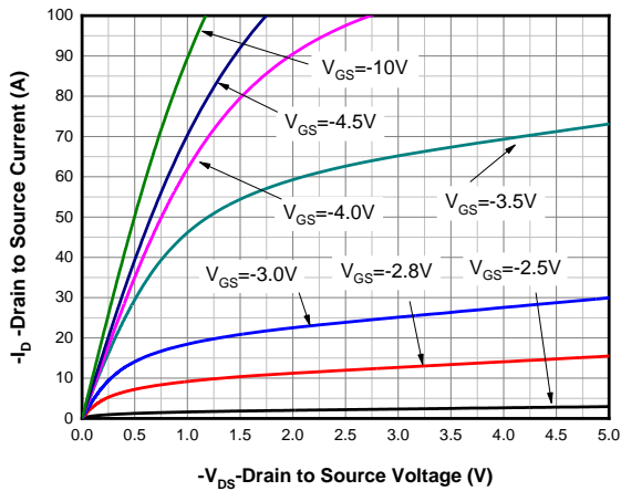
Output Characteristics (4)
