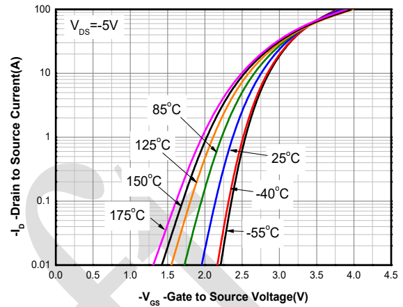
Transfer Characteristics (4)
